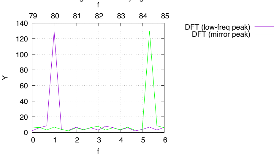
DFT of the generated noisy signal
